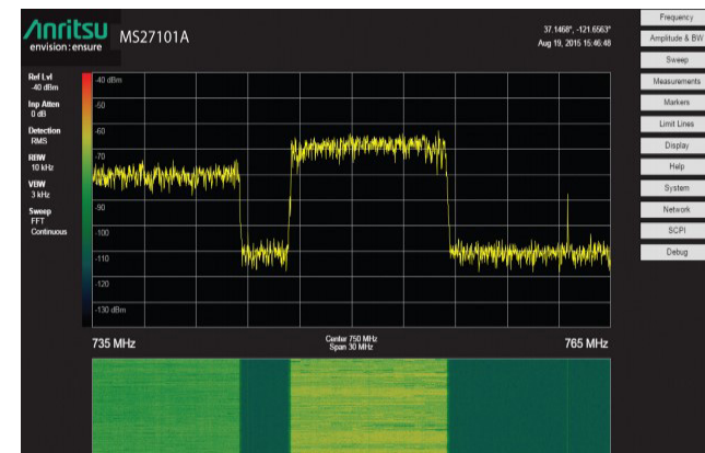
Spectrum and Spectrogram presented by Webserver Interface
